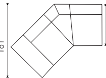
Terminal large L top view
